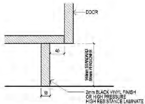
BASE DETAIL
