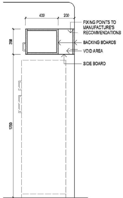
SECTION
